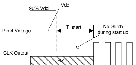
Figure 4. Startup Timing (OE/ST Mode) [9]
