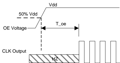
Figure 4. Startup Timing (OE/ST Mode) [9]
